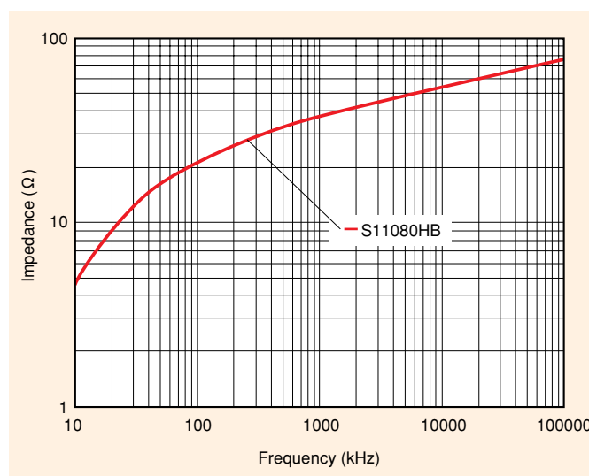
Figure 81. Frequency dependence of impedance for S11080HB
