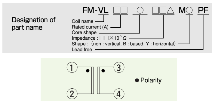
Figure 23. Circuit diagram
