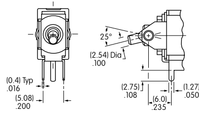
Vertical PC Mounting
