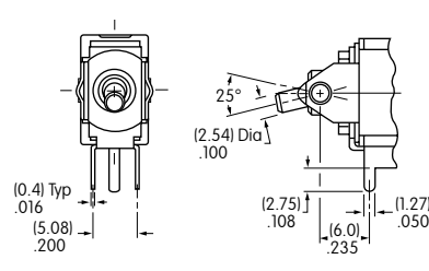
Vertical PC Mounting
