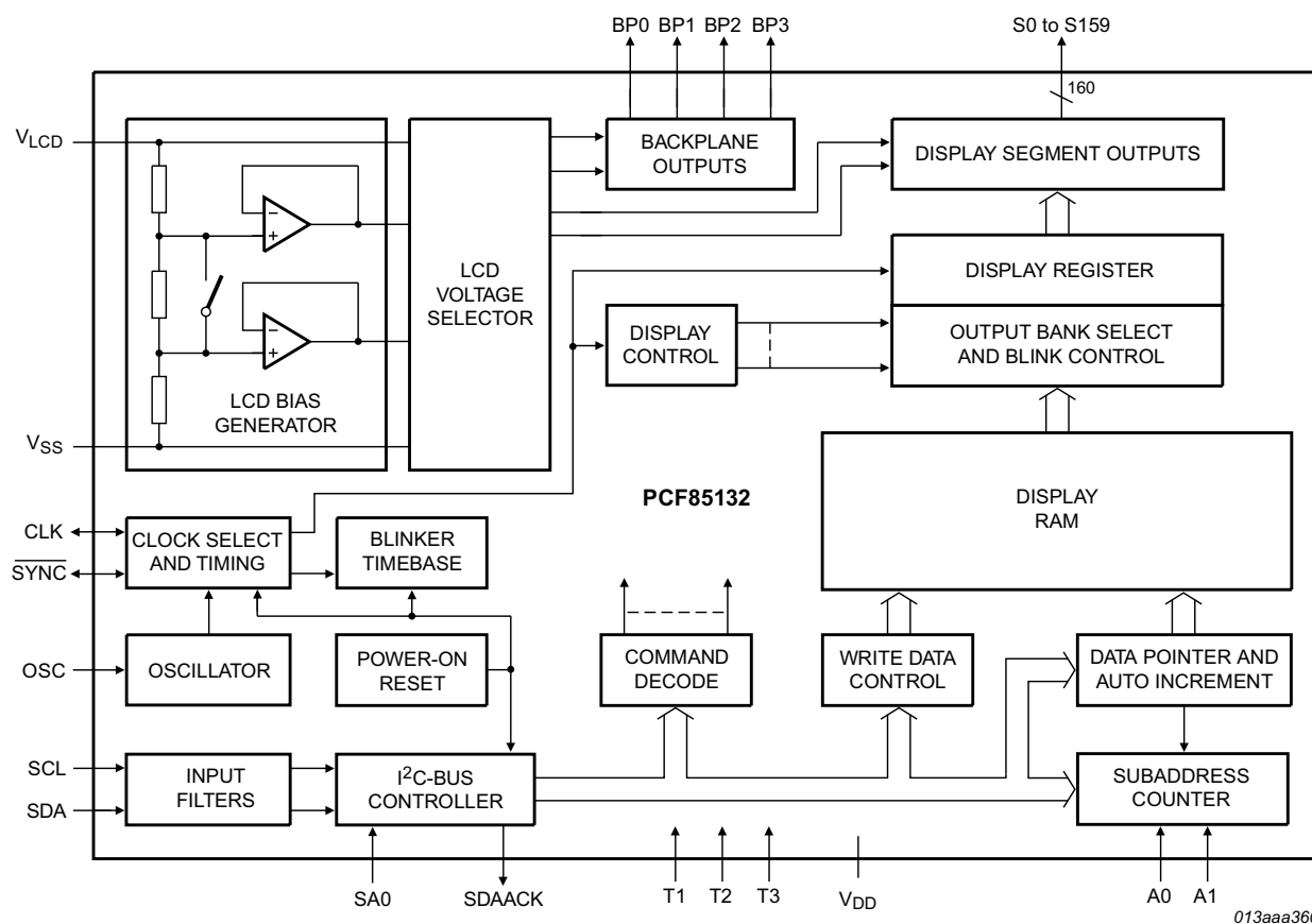
Fig 1. Block diagram of PCF85132
