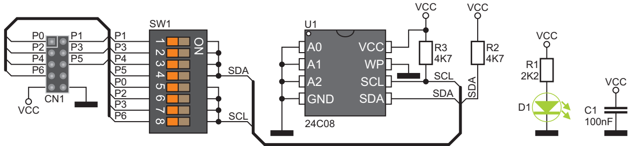
Figure 3-1: Connection schematic
