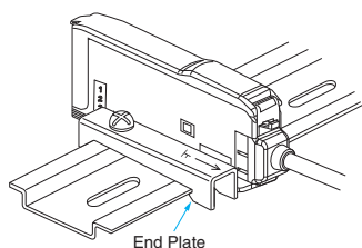
End Plate
