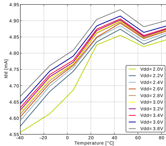
Figure 3.4. EM0 Current consumption while executing prime number calculation code from flash with HFRCO running at 14MHz
