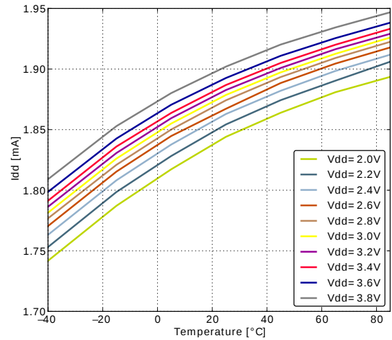
Figure 3.8. EM1 Current consumption with all peripheral clocks disabled and HFRCO running at 28MHz
