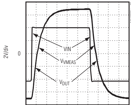
TRANSIENT RESPONSE FIMV MODE, RANGE D
