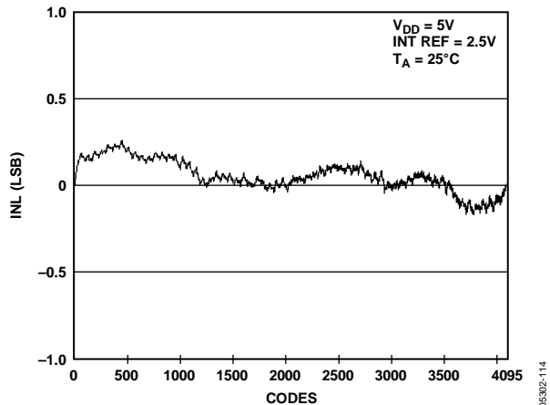
Figure 15. INL AD5628-2
