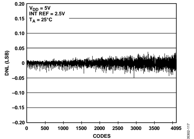
Figure 18. DNL AD5628-2
