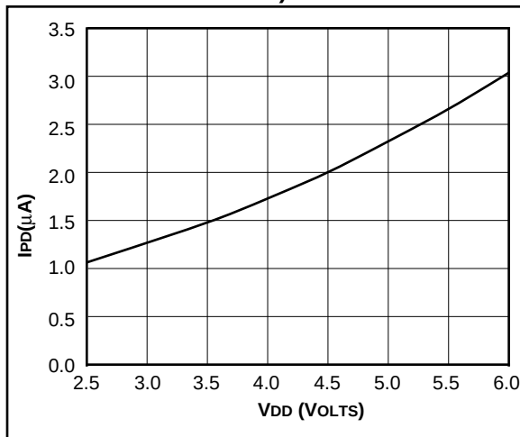
FIGURE 18-2: MAXIMUM I_{PD} vs. V_{DD} (WDT DISABLED, RC MODE -40°C TO +85°C)
