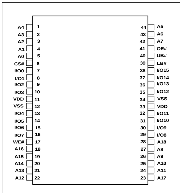
44-Pin TSOP-II, 1CS, No ERR
