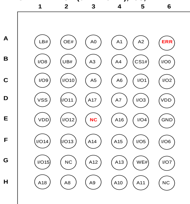
48-Pin mini BGA (6mm x 8mm), 1CS, ERR
