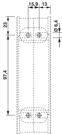
Dimensioned drawing
