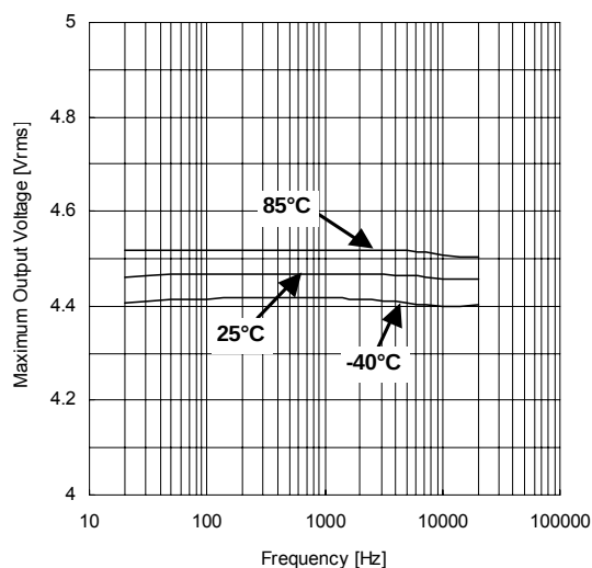
Maximum Output Voltage vs. Frequency V+/V- = ±7V, THD=1%
