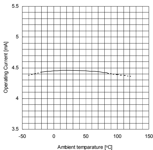
Operating Current vs. Ambient temperature V+/V- = ±7V, I CC
