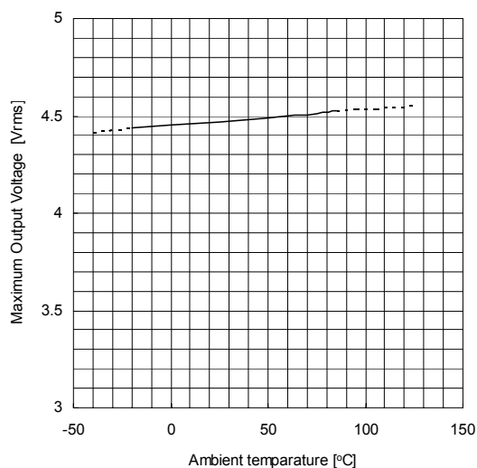
Maximum Output Voltage vs. Ambient temperature V+/V- = ±7V, THD=1%
