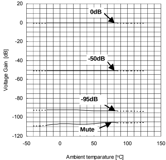
Voltage Gain vs. Ambient temperature V+/V- = ±7V, V in =0dBV, f=1kHz, R L =10kΩ
