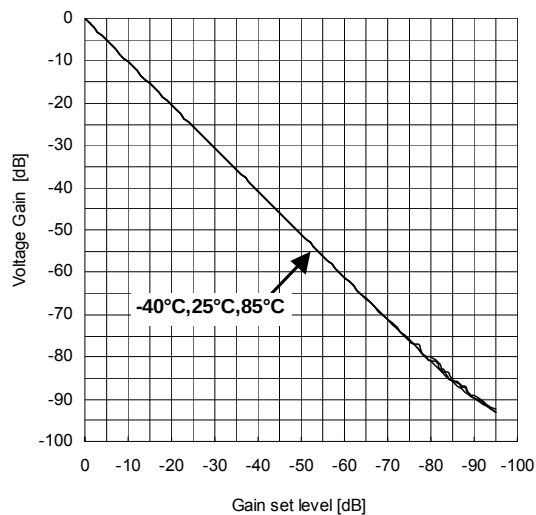
Voltage Gain vs. Gain set level V+/V- = ±7V, V in =0dBV, f=1kHz, R L =10kΩ
