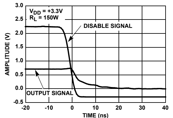
FIGURE 14. DISABLE TIME
