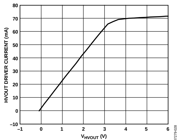
Figure 28. HVOOUT VH Current Limit; V_H = -0.1 V; V_{HVOOUT} Swept from -0.1 V to +6.0 V
