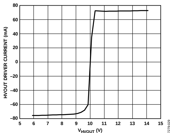
Figure 29. HVOOUT VHH Current Limit; V_{HH} = 10.0 V; V_{HVOOUT} Swept from -5.9 V to +14.1 V
