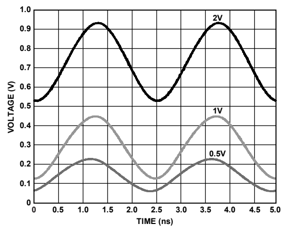
Figure 10. 400 MHz Driver Response; V_H = 0.5\text{ V} , 1.0\text{ V} , 2.0\text{ V} , V_L = 0.0\text{ V} ; 50\ \Omega Termination
