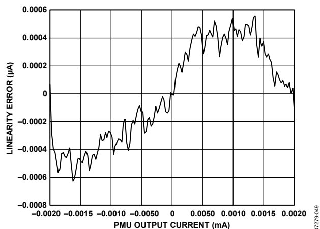
Figure 47. PMU Force Current Range E Linearity
