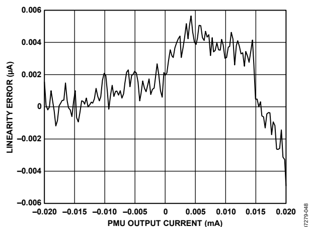
Figure 46. PMU Force Current Range D Linearity
