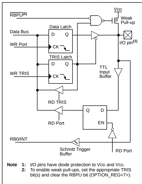
FIGURE 5-3: BLOCK DIAGRAM OF RB3:RB0 PINS
