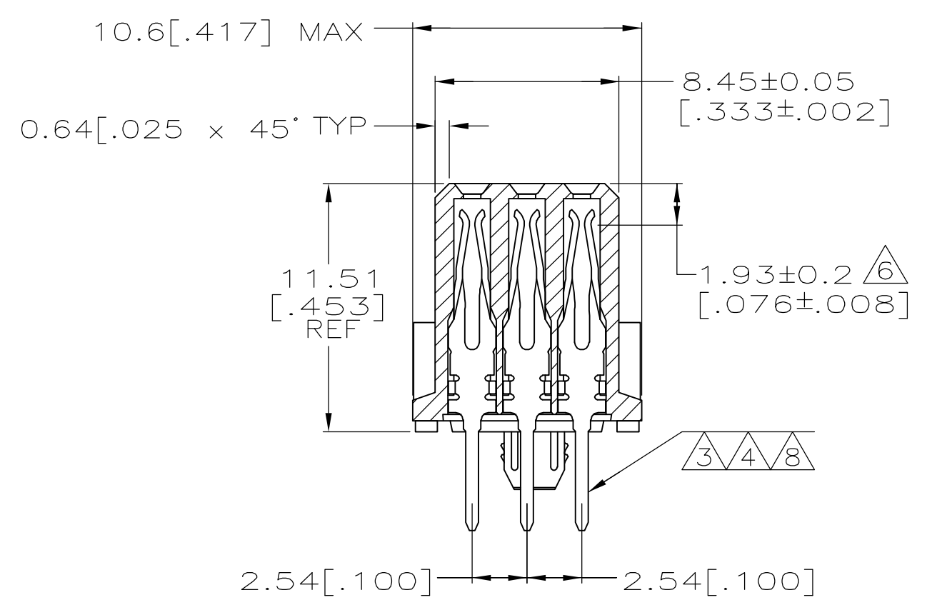
SECTION X-X
