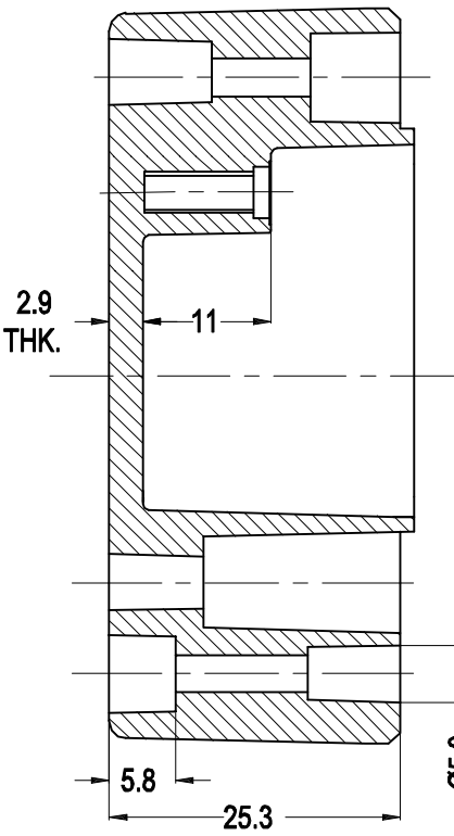
SECTION C-C
