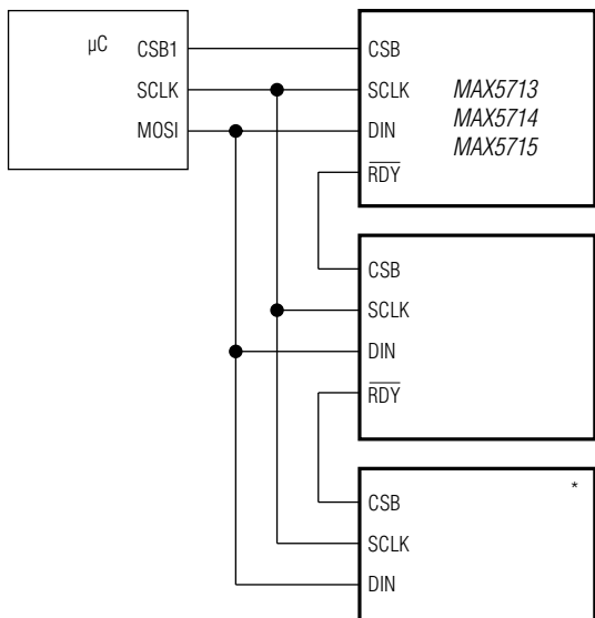
Figure 4. Typical SPI Daisy-Chain Application Circuit
