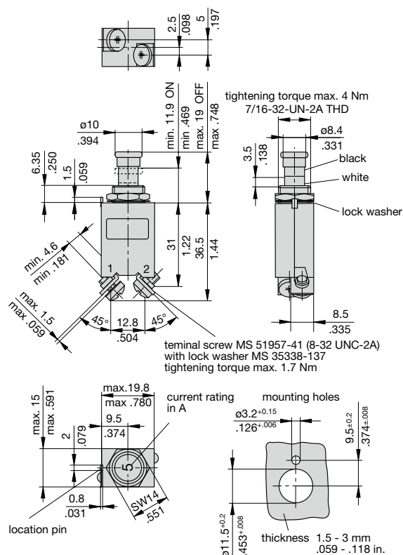
Dimensions 483-G533-J1M1-B2S0ZN (MS 3320)
