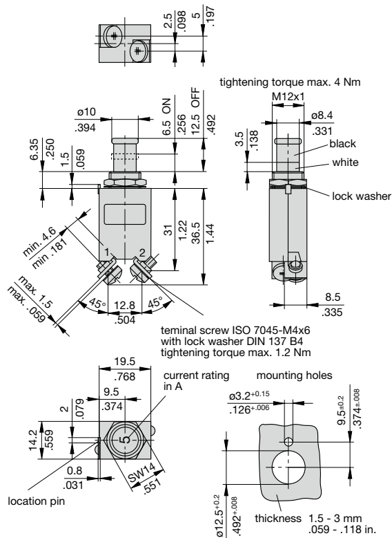
Dimensions 483-G411-K1M1-A1S0ZN (VG 95345 T06)
