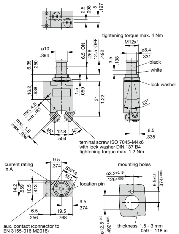
Dimensions 483-G111-K1M1-A1S1ZN (VG 95345 T06)
