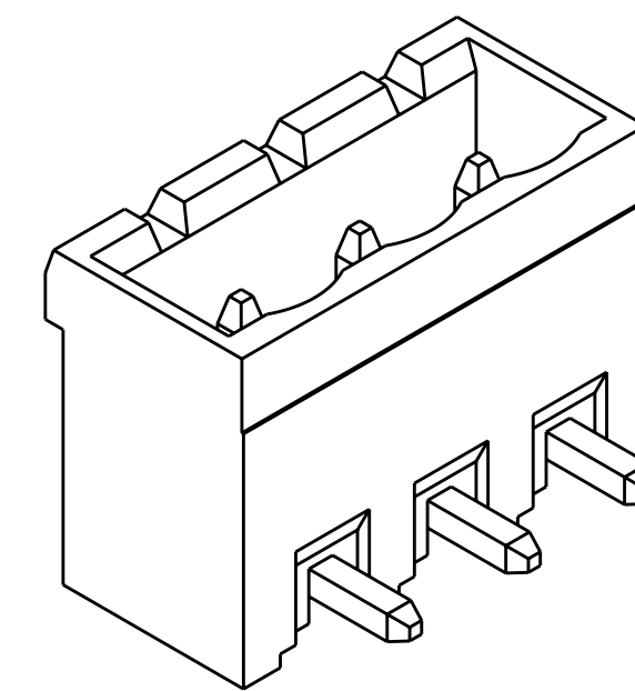
1546209-3 AS SHOWN
