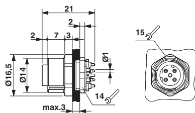
M12 flush-type connector
