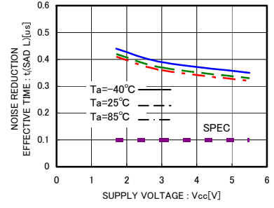
Fig.29 Noise reduction effective time t_t(SDA L)
