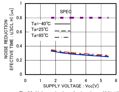
Fig.26 Noise reduction effective time t_t(SCL H)
