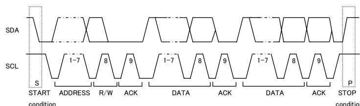
Fig.32 Data transfer timing
