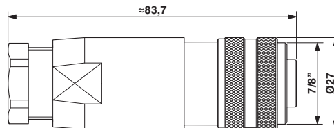
Dimensioned drawing
