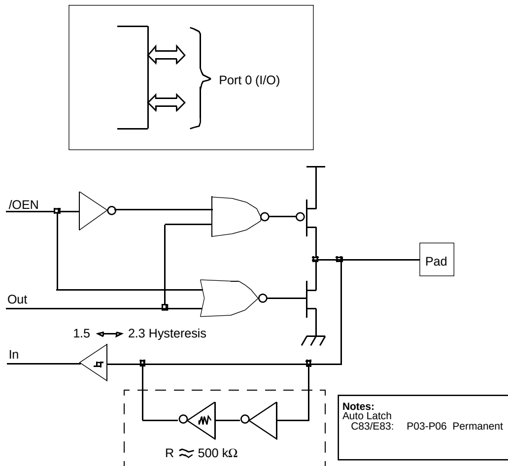
Figure 10. Port 0 Configuration
