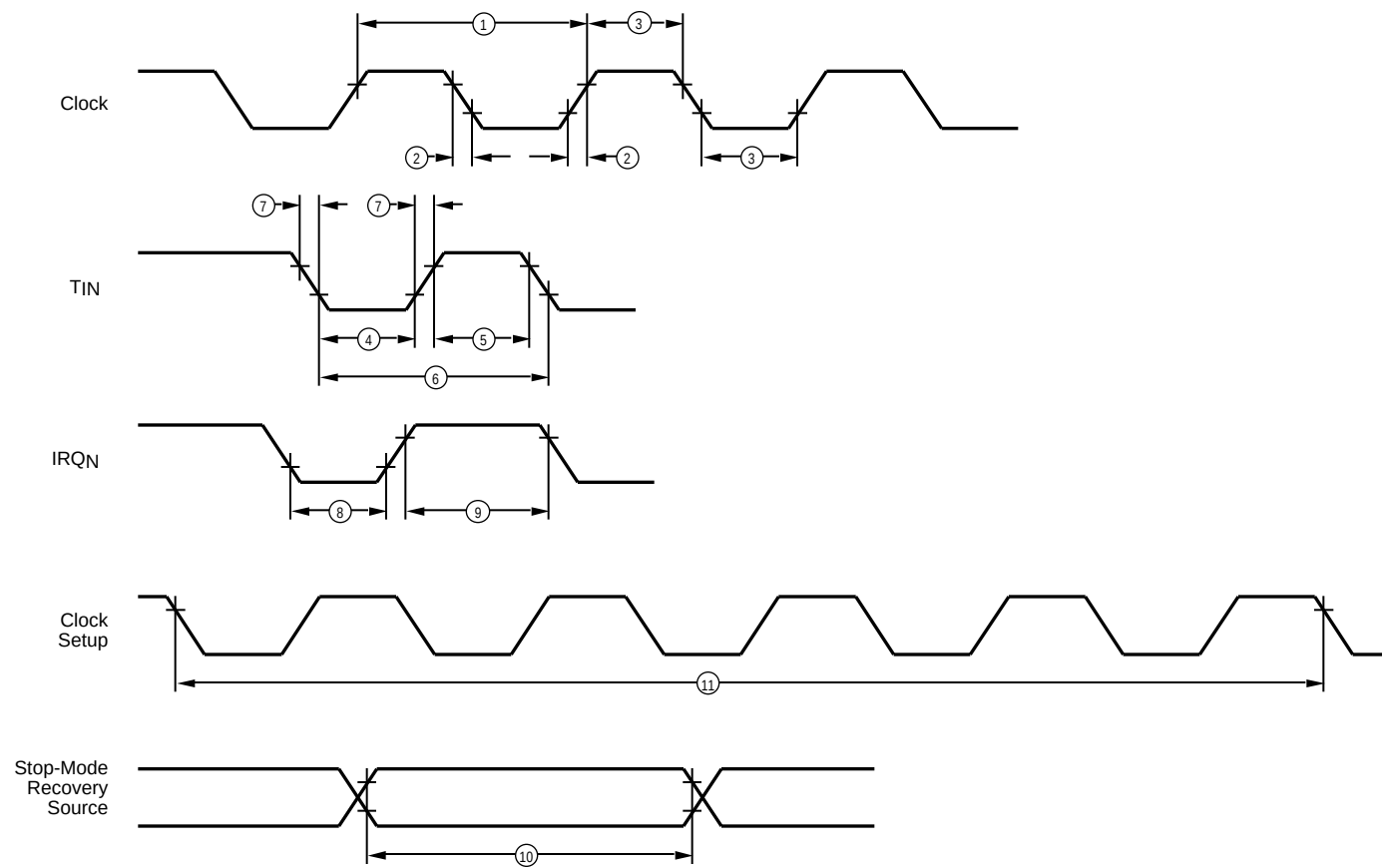
Figure 9. Additional Timing
