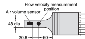
Figure 1: Wind Tunnel
