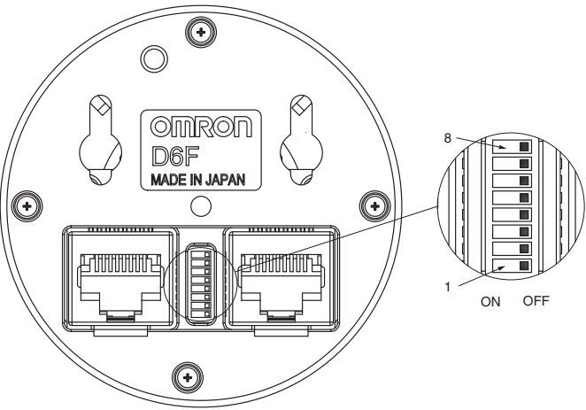
Fig. 3. DIP Switches
