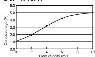
D6F-W01A1
