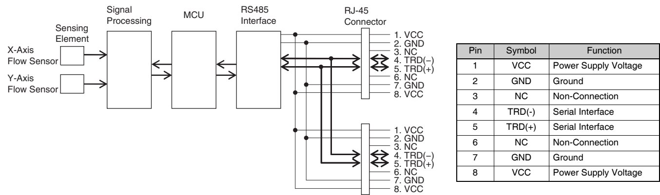
Fig. 2. Block Diagram
