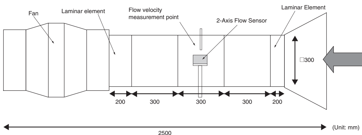
Fig. 1. Wind Tunnel
