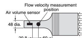
Figure 1: Wind Tunnel
