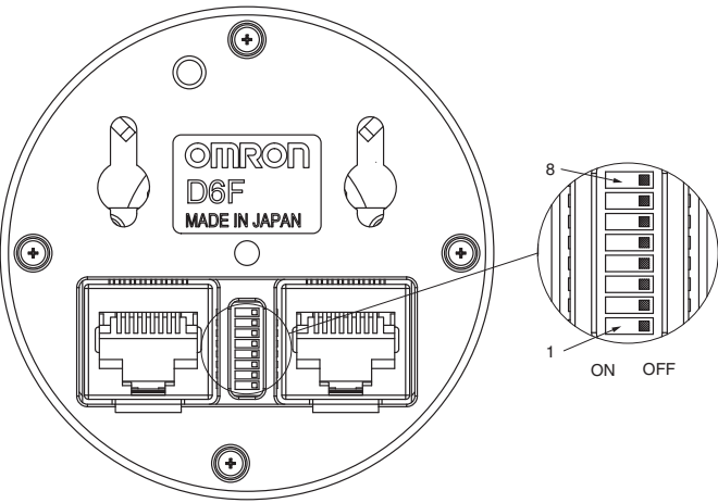
Fig. 3. DIP Switches
