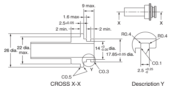
CROSS X-X
