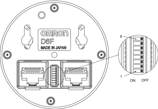
Fig. 3. DIP Switches
