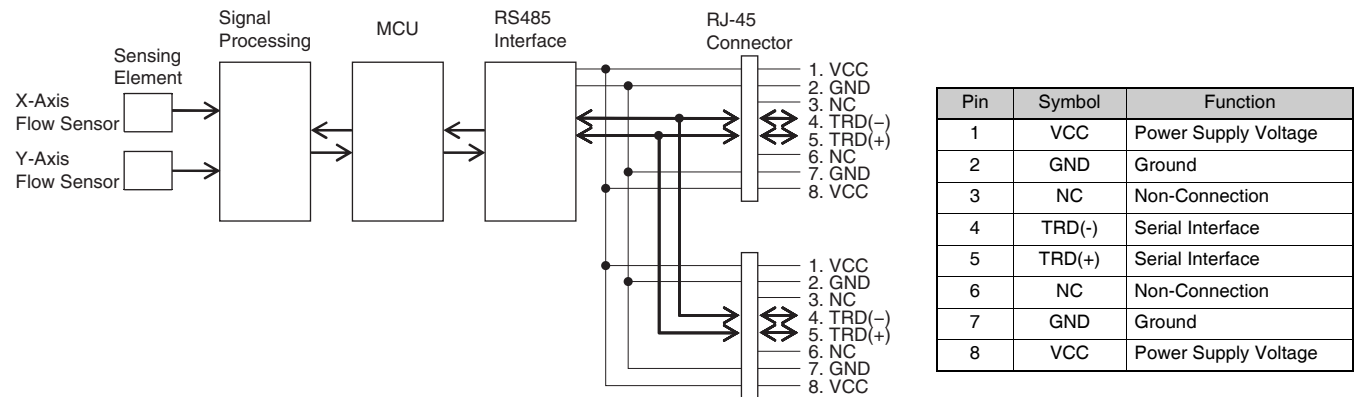
Fig. 2. Block Diagram
