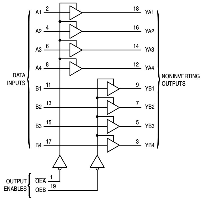
Figure 1. Logic Diagram
