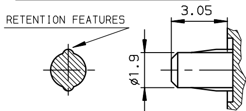
DETAIL OF FORCE-FIT PEGS
