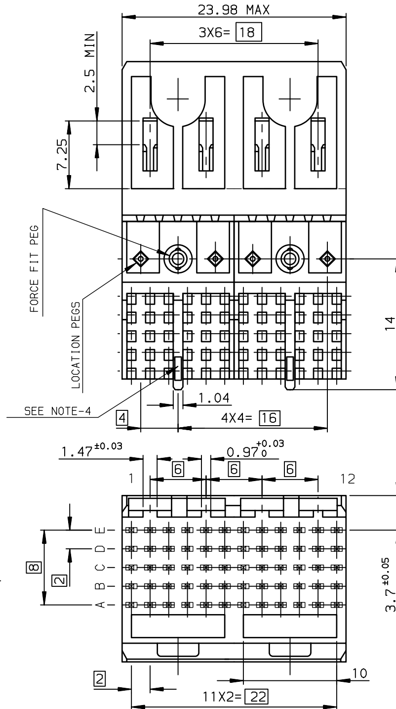
DETAIL-1: PRESS-FIT
