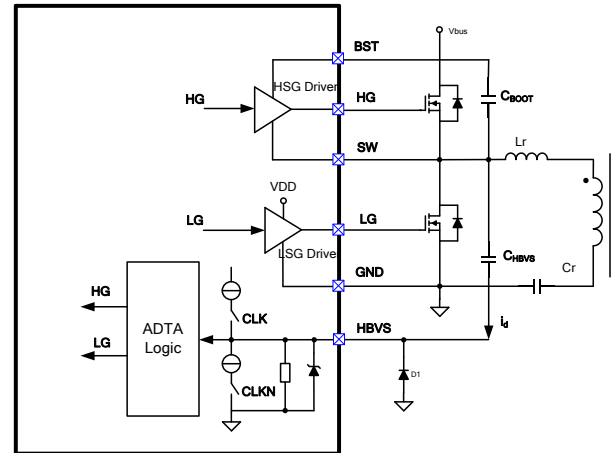
Figure 5: Block Diagram of ADTA
