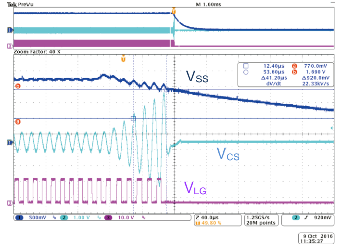
Figure 14: SCP Waveform
