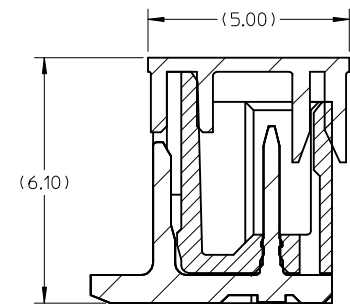
SECTION A-A (WITH CAP)
