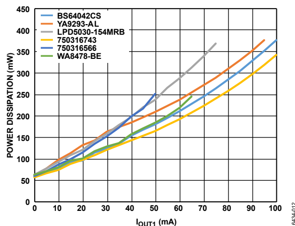
Figure 13. Power Dissipation using Various Transformers, T_A = +25^\circ\text{C} , V_{INP} = +24\text{ V} , V_{OUT1} = +24\text{ V} , V_{OUT2} = +5.15\text{ V} , I_{OUT2} = +7\text{ mA} , V_{OUT3} = -15\text{ V} , I_{OUT3} = -0.3\text{ mA}
