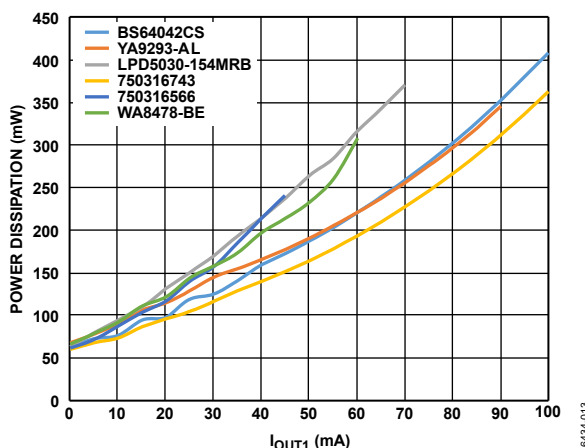
Figure 14. Power Dissipation using Various Transformers, T_A = +125^\circ\text{C} , V_{INP} = +24\text{ V} , V_{OUT1} = +24\text{ V} , V_{OUT2} = +5.15\text{ V} , I_{OUT2} = +7\text{ mA} , V_{OUT3} = -15\text{ V} , I_{OUT3} = -0.3\text{ mA}
