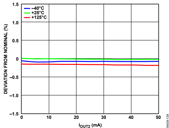
Figure 34. Buck Regulator Load Regulation Across Temperature, V_{OUT1} = 24\text{ V} , V_{OUT2} = 5.15\text{ V} , Nominal = V_{OUT2} at 10\text{ mA } I_{OUT2}
