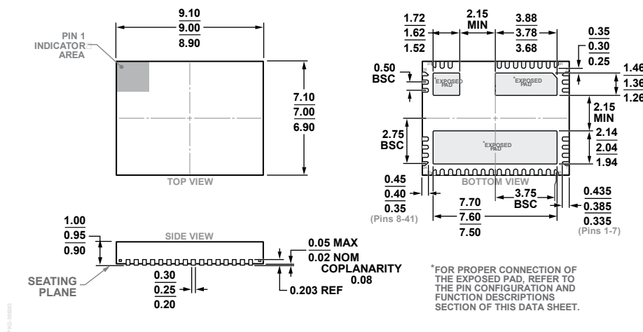
Figure 78. 41-Lead Lead Frame Chip Scale Package [LFCS] 9 mm × 7 mm Body and 0.95 mm Package Height (CP-41-1)
