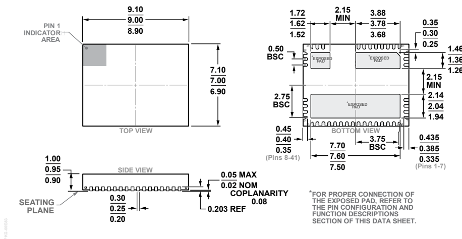
Figure 78. 41-Lead Lead Frame Chip Scale Package [LFCSPP] 9 mm × 7 mm Body and 0.95 mm Package Height (CP-41-1)
