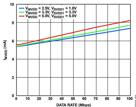
Figure 48. MVDD Supply Current ( I_{MVDD} ) per SPI Input vs. Data Rate at Various Supply Voltages, \overline{MSS} Is Low, Clock Signal Applied on Single SPI Channel, Other Input Channels Tied Low
