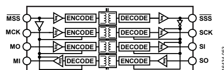
Figure 67. iCoupler Gating
