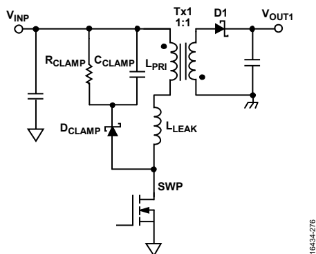
Figure 72. Resistor, Capacitor, Diode Clamp
