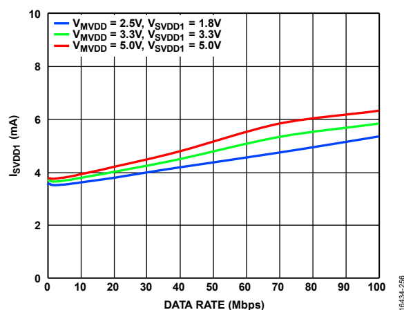
Figure 51. SVDD1 Supply Current ( I_{SVDD1} ) per SPI Input vs. Data Rate at Various Supply Voltages, \overline{SSS} Is Low, Clock Signal Applied on Single SPI Channel, Other Input Channels Tied Low
