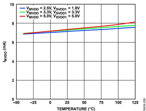
Figure 53. I_{MVDD} vs. Temperature at Various Supply Voltages, \overline{MSS} Is Low, Data Rate = 10 Mbps on All SPI Channels
