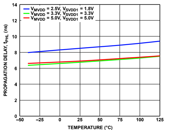
Figure 57. SPI Channels Propagation Delay ( t_{PLH} ) vs. Temperature at Various Supply Voltages
