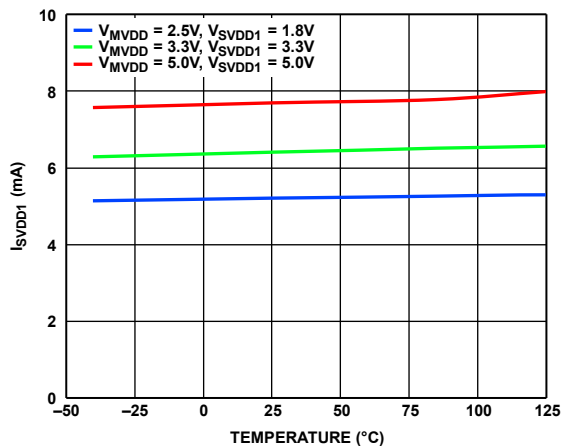
Figure 56. I_{SVDD1} vs. Temperature at Various Supply Voltages, \overline{SSS} Is Low, Data Rate = 10 Mbps on All SPI Channels
