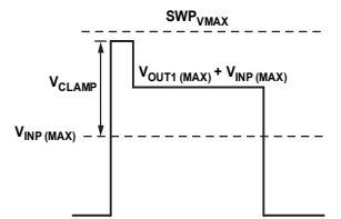
Figure 74. Clamping Waveform
