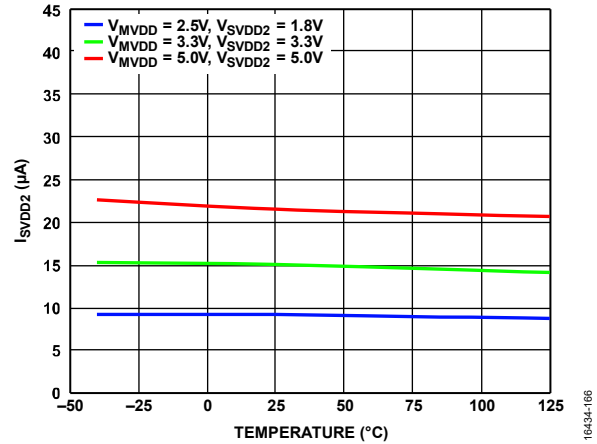
Figure 62. I_{SVDD2} vs. Temperature at Various Supply Voltages, \overline{MSS} Is Low, Data Rate = 40 kbps on All GPIO Channels
