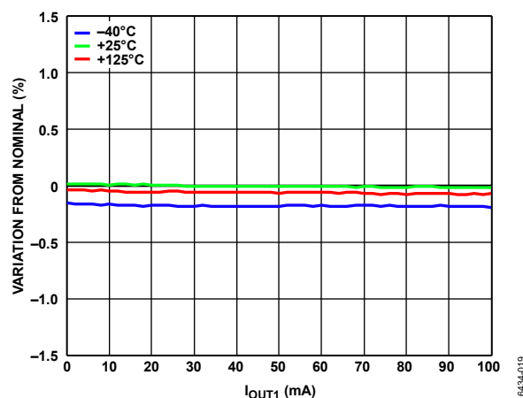
Figure 20. Flyback Regulator Load Regulation Across Temperature, V_{INP} = 24\text{ V} , V_{OUT1} = 21\text{ V} , Nominal = V_{OUT1} at 20 mA Load
