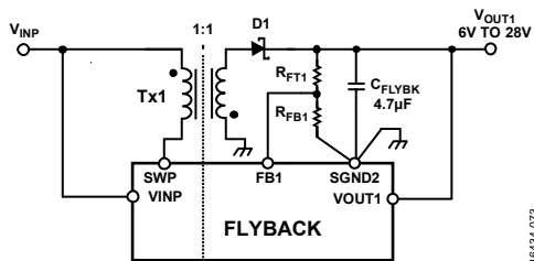
Figure 70. Flyback Regulator Output Voltage Setting
