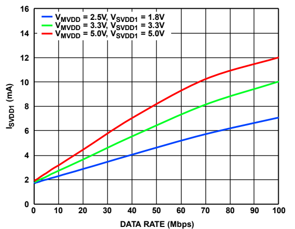
Figure 55. I_{SVDD1} vs. Data Rate at Various Supply Voltages, \overline{SSS} Is Low, Clock Signal Applied on Single SPI Channel, Other Input Channels Tied Low
