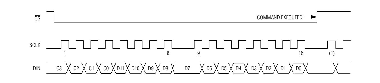
Figure 2. Serial-Interface Signals
