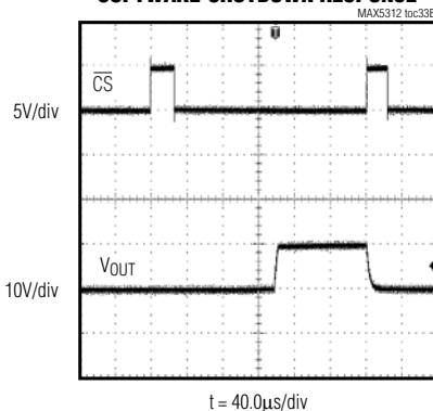
BIPOLAR SOFTWARE-SHUTDOWN RESPONSE
