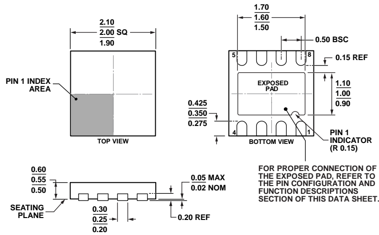
Figure 21. 8-Lead Lead Frame Chip Scale Package [LFCSPP] 2.00 mm × 2.00 mm Body, and 0.55 mm Package Height (CP-8-10) Dimensions shown in millimeters
