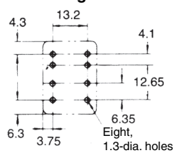
Mounting Holes
