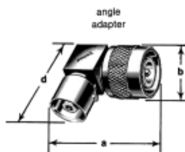
Angle Adapters 82-535
