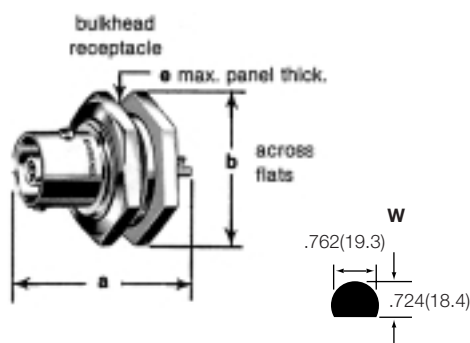
Bulkhead Receptacles 82-515
