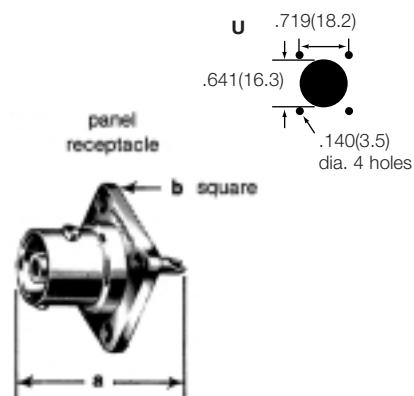
Panel Receptacles 82-504
