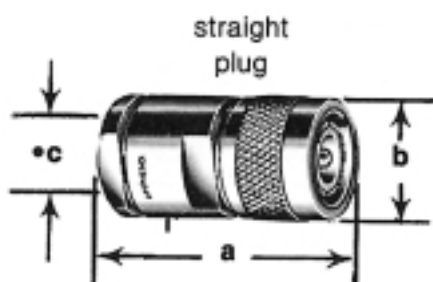
Straight Plug 82-530 82-532
