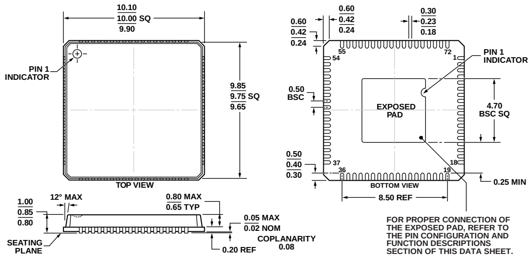
Figure 43. 72-Lead Lead Frame Chip Scale Package [LFCSP_VQ] 10 mm x 10 mm, Very Thin Quad (CP-72-1)
