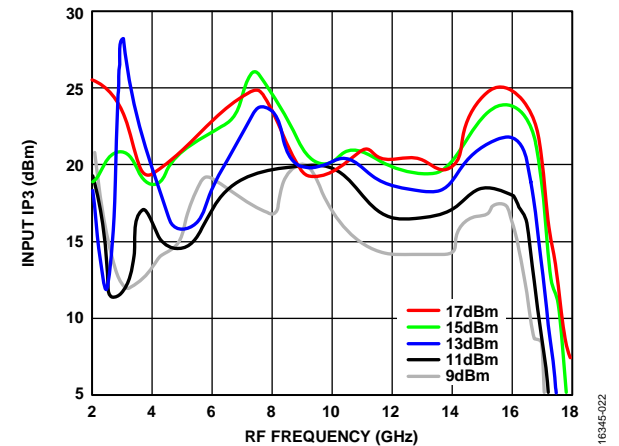
Figure 21. Input IP3 vs. RF Frequency over LO Drive at f_{IF} = 1500 MHz, T_A = 25^\circ\text{C}
