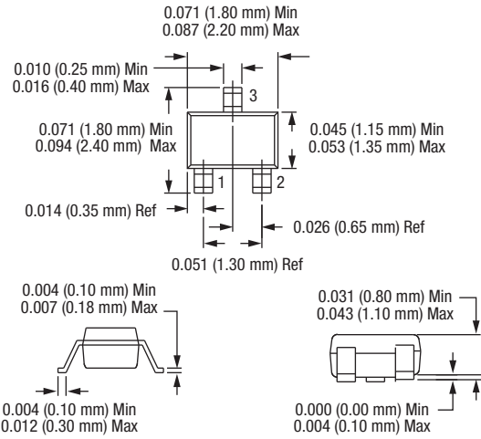
Dimensions are in inches (millimeters shown in parentheses) 200047-005
