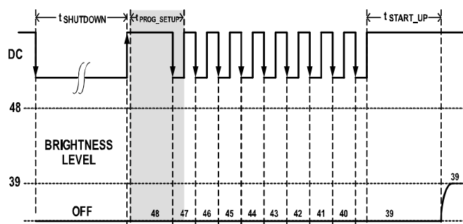
Figure 16. Presetting Timing
