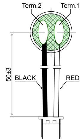
BOTTOM VIEW
