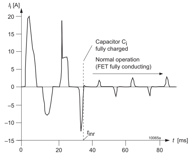
Fig. 31 Inrush current for LS models with option E (AC supply) V_i = 230 \text{ VAC} , f_i = 50 \text{ Hz} , P_o = P_{o \text{ nom}}
